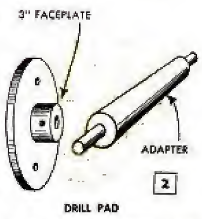
In live drilling, pictured in the photos above and below, the drill usually is held in a geared chuck and driven by the lathe headstock. Flat work is supported by a pad as in the lower views. Note wooden facing
